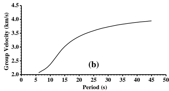
Fig. 9. (a) Shear velocity distribution of the initial model (as listed in Table 5). (b) Theoretical group velocity obtained from the initial model listed in Table 5, by means of forward modelling.
